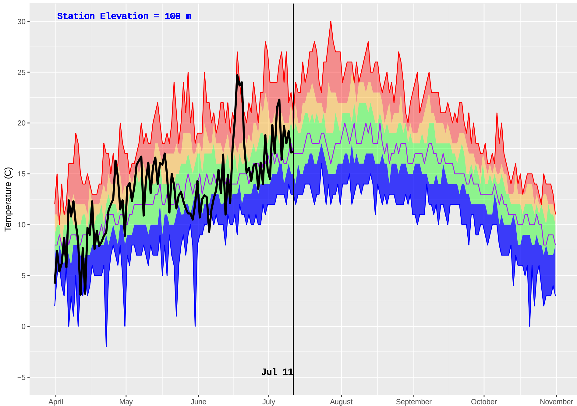
HONNA (93) : Historical (1986–2016) and Current (2018) Noon Temperature
