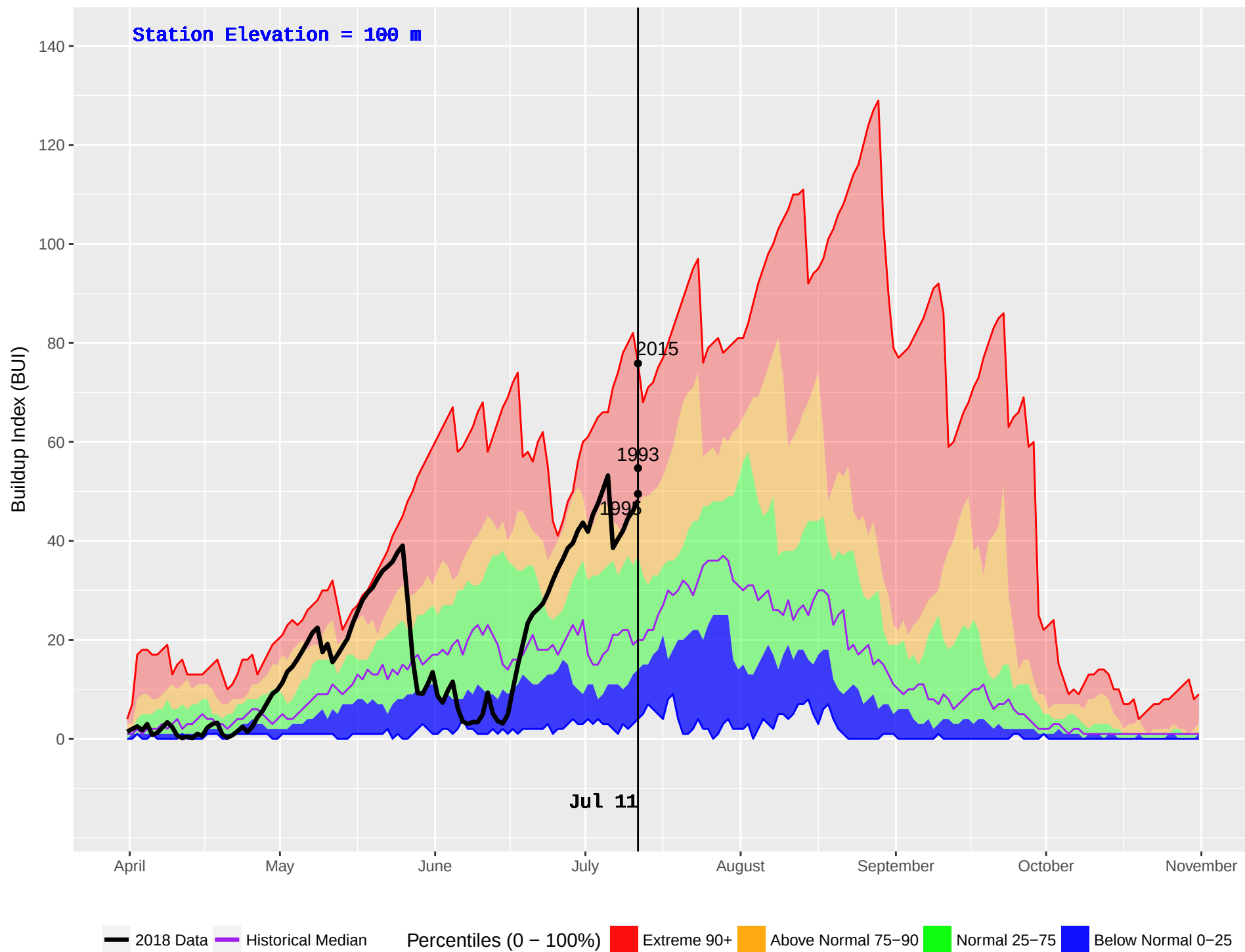
HONNA (93) : Historical (1986–2016) and Current (2018) Noon Buildup Index (BUI)
